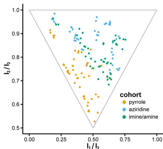
Figure 2. Principal moment-of-inertia analysis of newly synthesized compounds. Individual points indicate the location of a given conformer (up to five conformers per compound) in PMI space, as defined by the ratios of their computed principal moments of inertia ( I_1 < I_2 < I_3 ). Points near the top-left corner indicate one-dimensional “rod-like” character, points near the bottom indicate two-dimensional “disc-like” character, and points near the top-right corner indicate three-dimensional “sphere-like” character.
