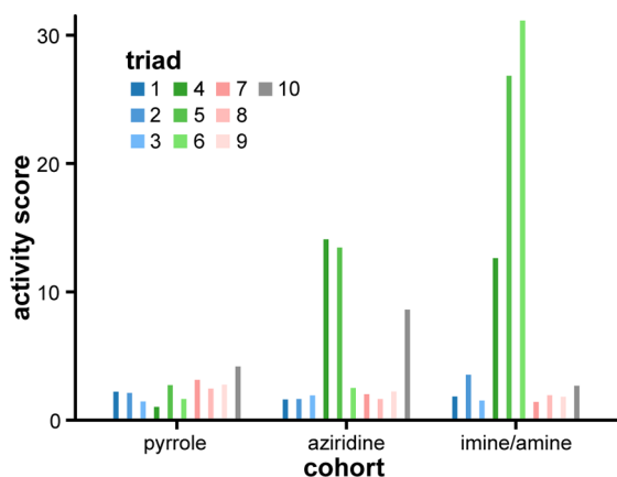
Figure 4. Bar graph of compound activities reveals contributions from both skeleton and appendage identities. Activity scores for each compound were averaged across replicates of all concentrations. Compounds are grouped by cohorts and colored by triads, with differing shades of a given color indicating a shared electron-withdrawing group (blue, acetyl; green, nitrile; salmon, ester; gray, amide). Representing the data in this format emphasizes the influence of both skeletons and appendages on biological activity. In particular, the combination of a nitrile appendage on an aziridine or imine/amine skeleton yields highly active compounds.
