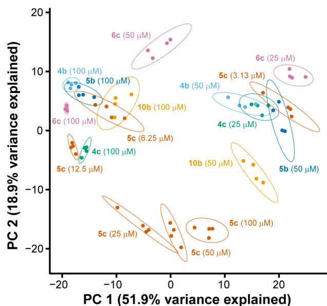
Figure 6. Principal component analysis of compound-induced changes in cell morphology illuminates differences in MoAs of active compounds. Tight clusters of treatment replicates, represented by individual points and encircled by ellipses, demonstrate the high reproducibility of compound-induced changes in cell morphology. Analyzing biological annotation data across various compound concentrations provides greater resolution with regard to compound MoA. Points and ellipses (drawn at 95% confidence intervals) are colored according to compound identities.
