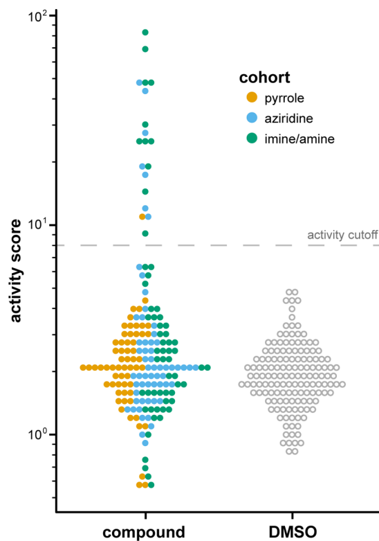
Figure 3. Dot plot depicting compound activities compared to DMSO alone. Activity scores describe the degree to which compound-induced morphological changes are distinct from those induced by DMSO alone and are calculated according to the distance metric described by Mahalanobis. 24 Each point represents a single compound-treatment condition (compound A, concentration X), averaged across four replicates. The dashed line indicates the cutoff at which compound treatment conditions were considered “active”.
