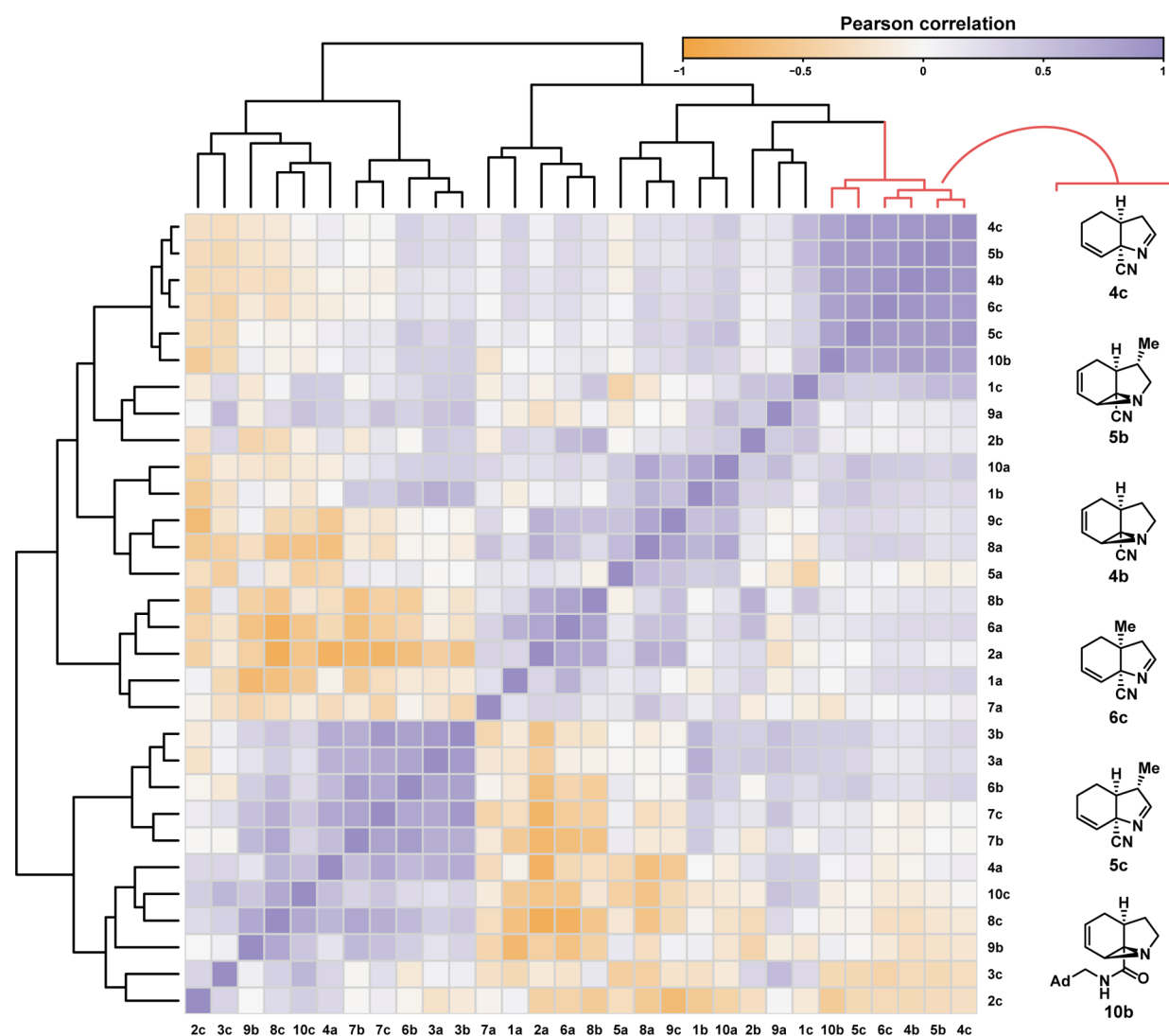
Figure 5. Heat map showing relationships of compounds (compound vs compound) based on the similarities of their biological profiles. Biological profiles are compared using pairwise Pearson correlation coefficients, calculated from the patterns of cell morphology changes (1140 total features) induced by compound treatment (average of six concentrations, each in quadruplicate). Structures of the six most highly correlated compounds (red clade in top dendrogram) are shown to the right of the heat map.
