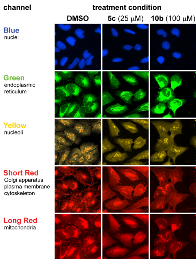
Figure 7. Actual images of vehicle-, compound 5c- (25 \mu M), and compound 10b-treated (100 \mu M) cells observed across five channels. The images reinforce that the two highly active compounds depicted have distinct effects on cell morphology, despite their membership in a distinct clade when compared to all other compounds (cf., Figure 5). The discrete morphological features best visualized in each channel are listed below the channel names.
